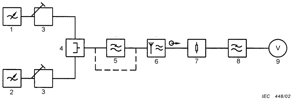
Figure 2 – Audio power output measurement
